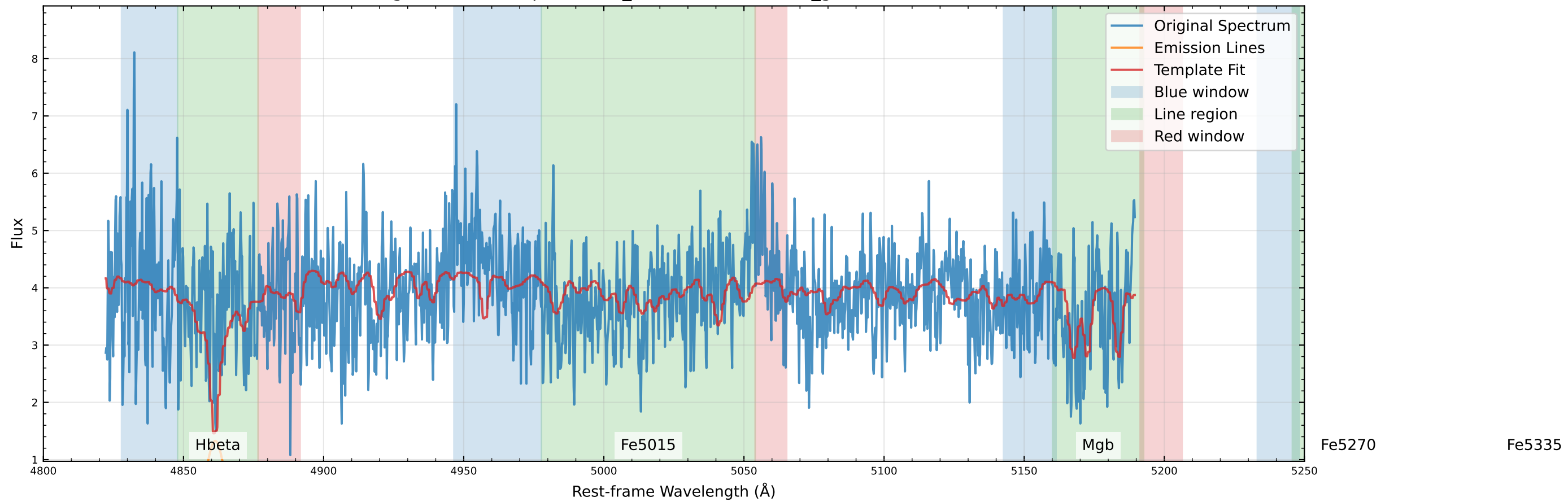
Original Data Comparison (v_star=-109.2 km/s, v_gas=-105.5 km/s)
