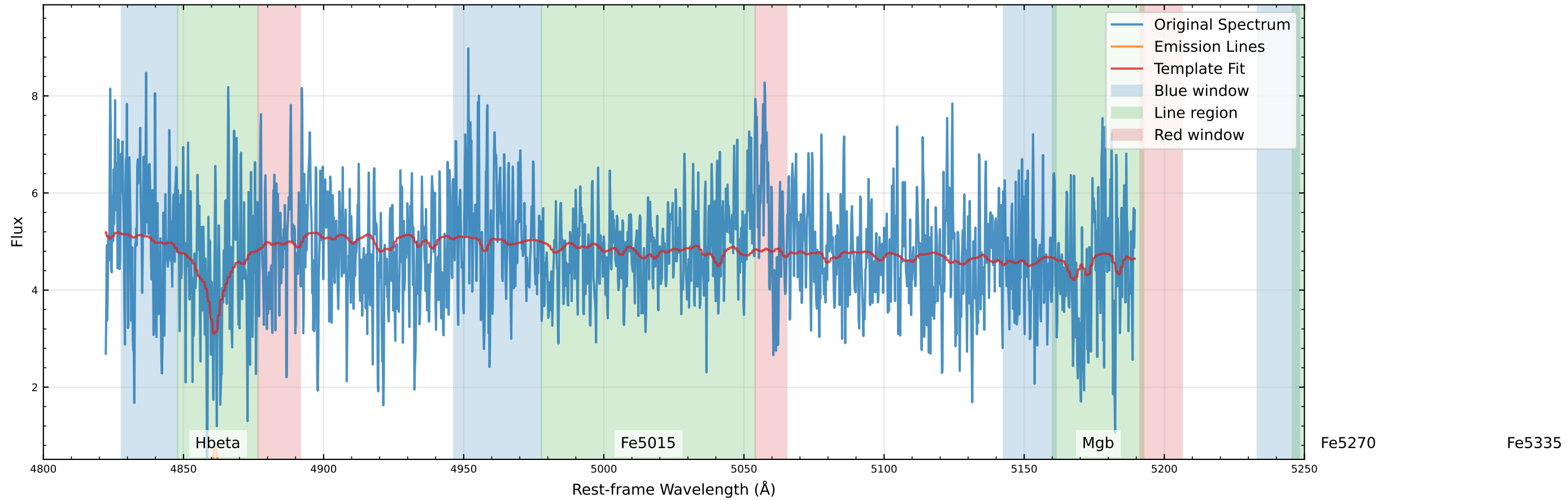
Original Data Comparison (v_star=-48.5 km/s, v_gas=-37.0 km/s)
