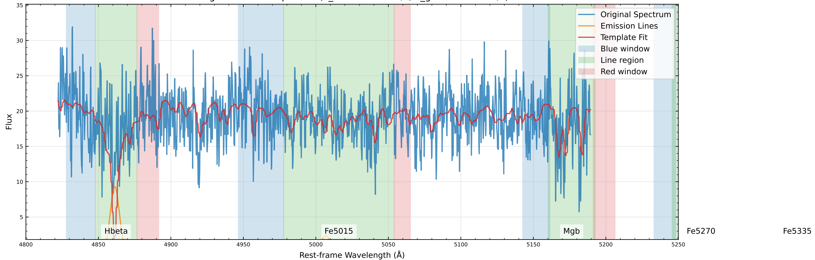
Original Data Comparison (v_star=-59.7 km/s, v_gas=-111.7 km/s)
