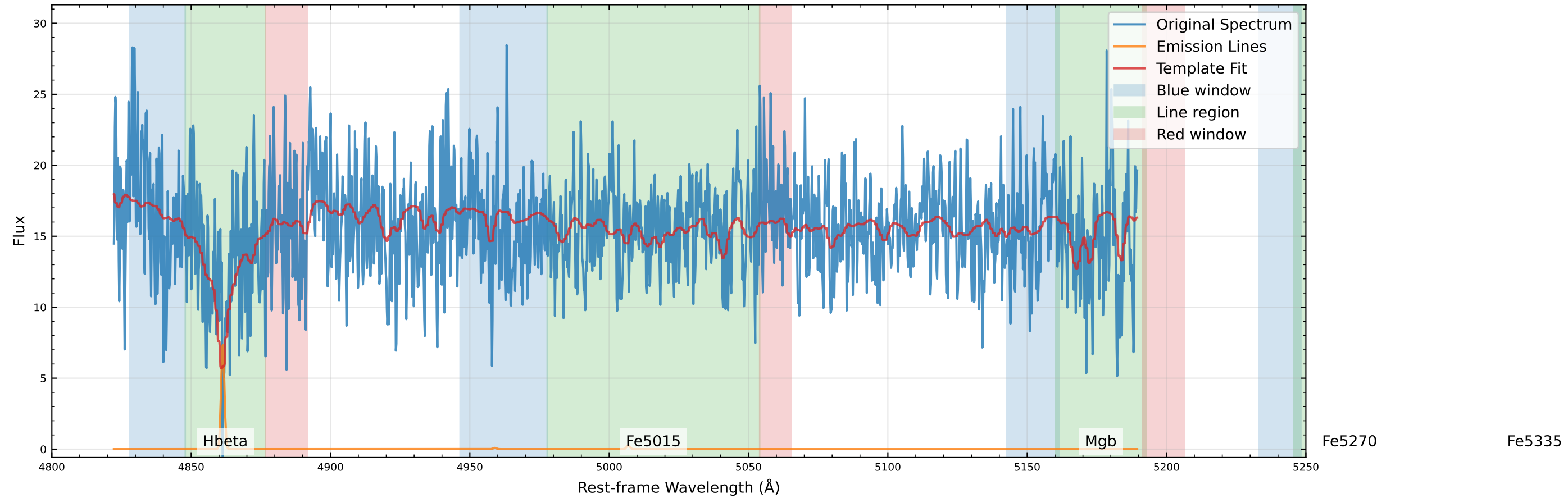
Original Data Comparison (v_star=-14.3 km/s, v_gas=-71.0 km/s)
