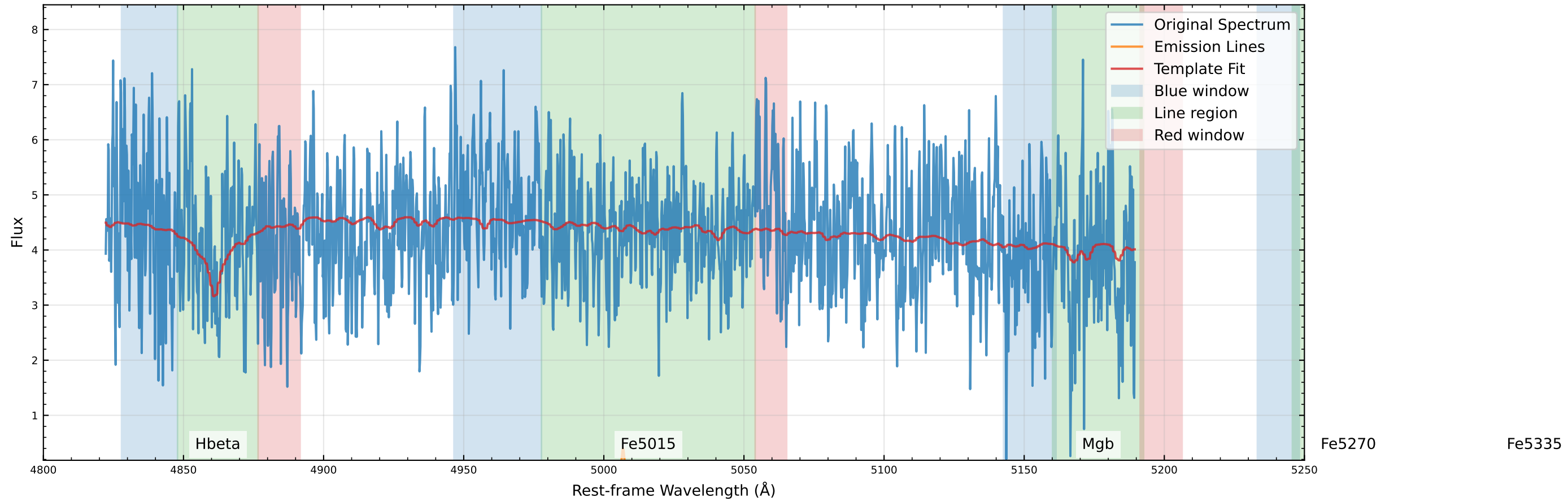
Original Data Comparison (v_star=16.8 km/s, v_gas=20.4 km/s)
