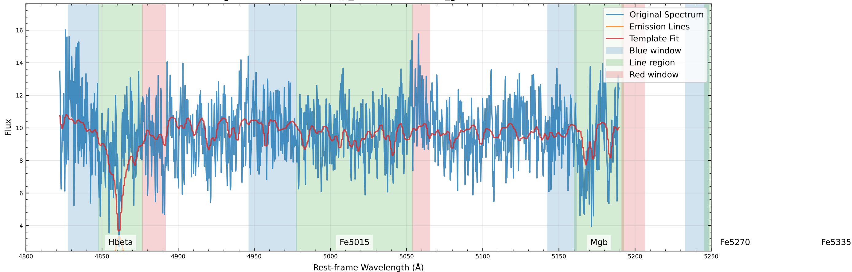
Original Data Comparison (v_star=-35.6 km/s, v_gas=87.5 km/s)
