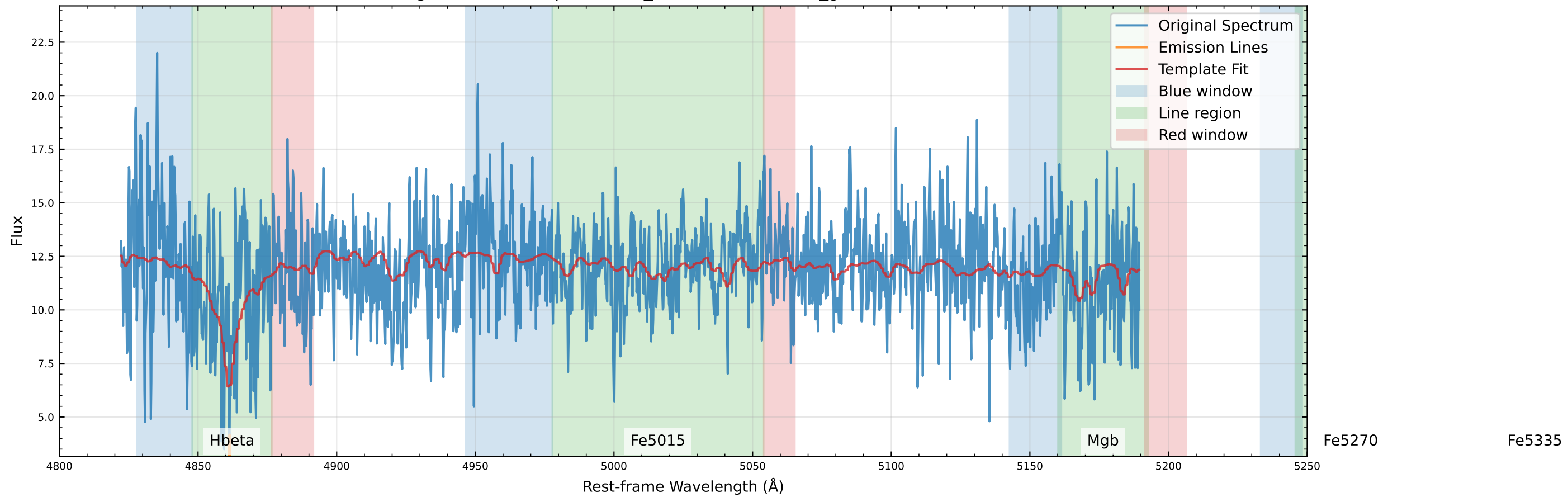
Original Data Comparison (v_star=-16.8 km/s, v_gas=-56.5 km/s)
