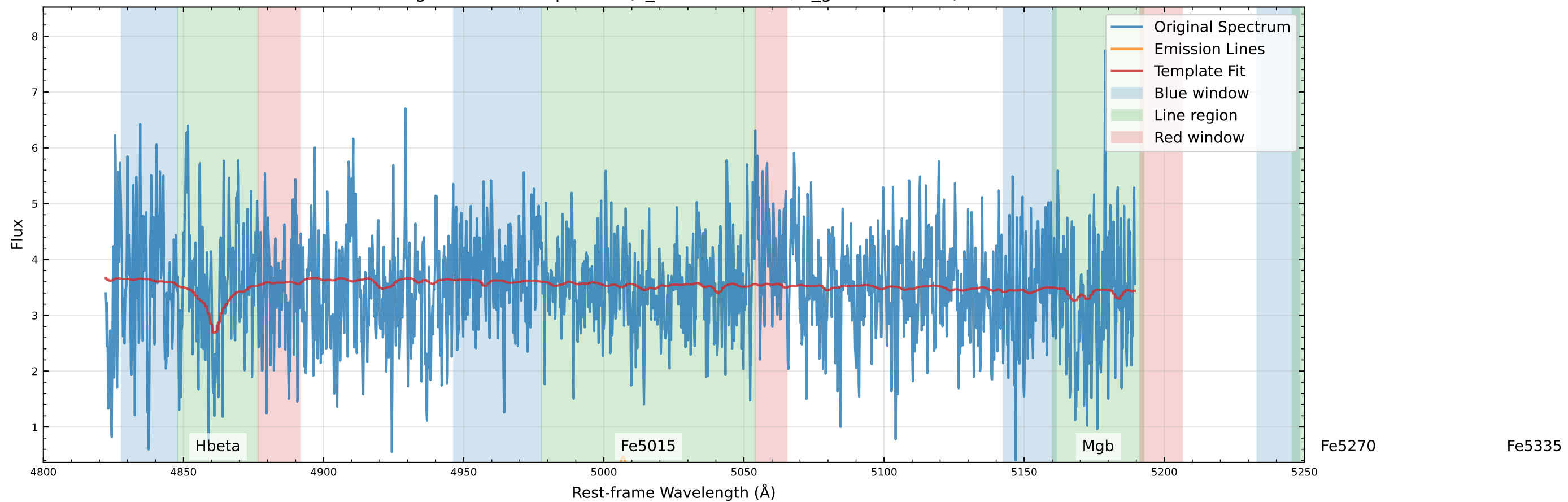
Original Data Comparison (v_star=-3.9 km/s, v_gas=-2.7 km/s)
