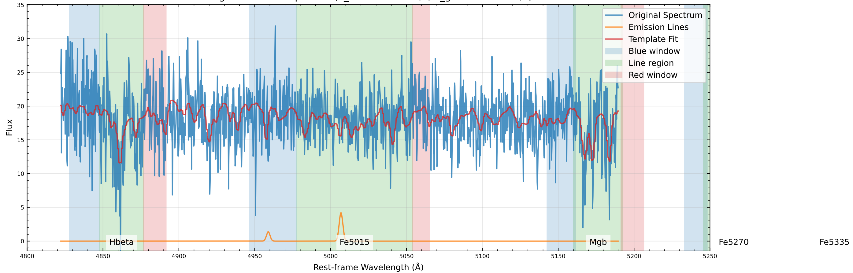
Original Data Comparison (v_star=-18.4 km/s, v_gas=-129.1 km/s)
