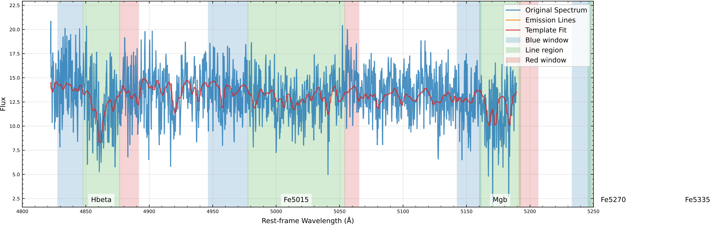
Original Data Comparison (v_star=-34.4 km/s, v_gas=-32.4 km/s)
