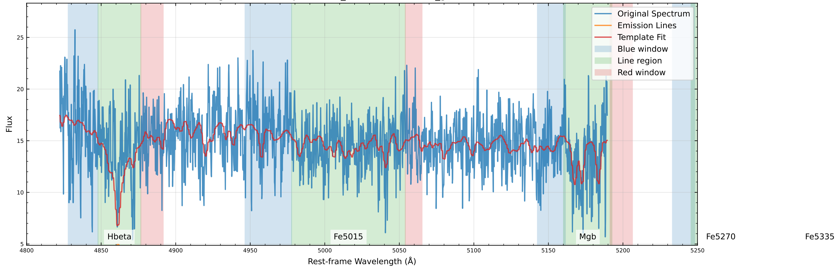
Original Data Comparison (v_star=-18.0 km/s, v_gas=-45.0 km/s)
