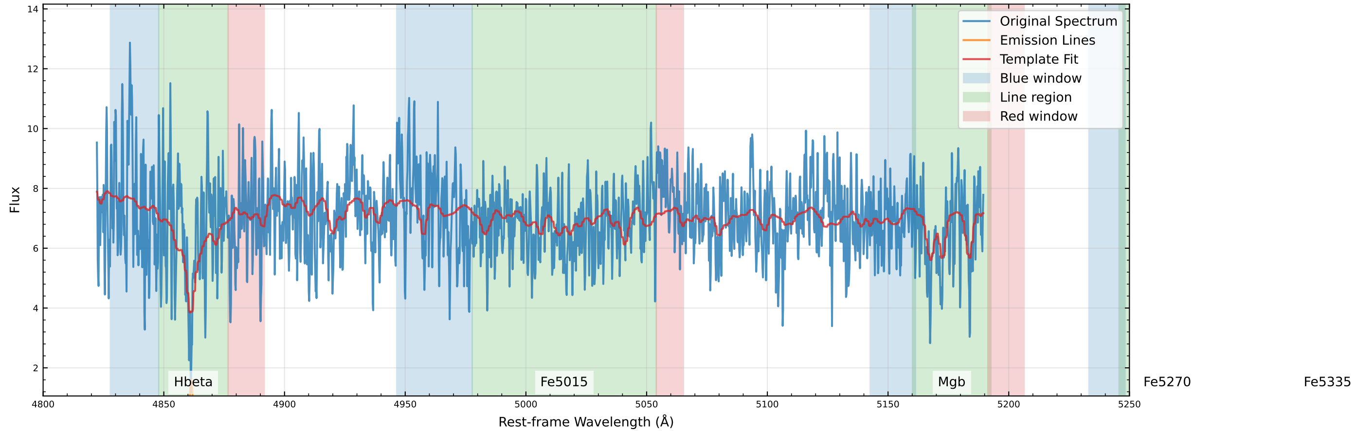
Original Data Comparison (v_star=-23.7 km/s, v_gas=128.3 km/s)
