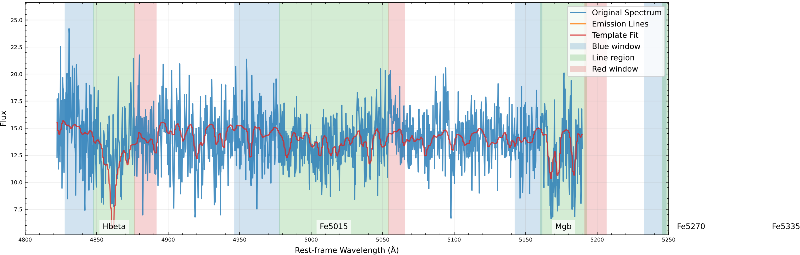
Original Data Comparison (v_star=8.9 km/s, v_gas=3.3 km/s)
