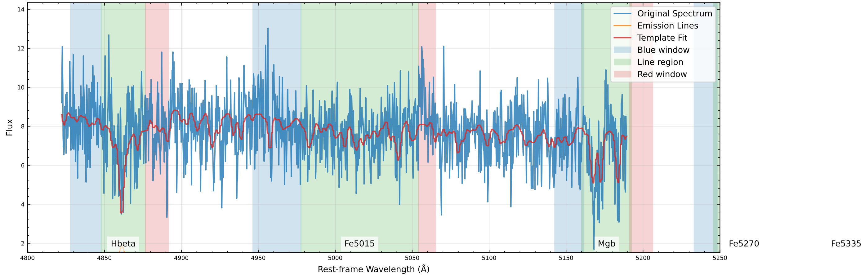
Original Data Comparison (v_star=19.8 km/s, v_gas=122.8 km/s)
