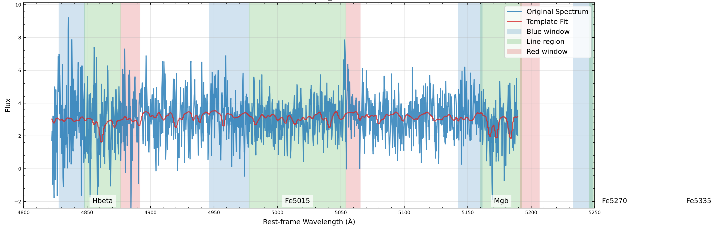
Original Data Comparison (v_star=-130.5 km/s)
