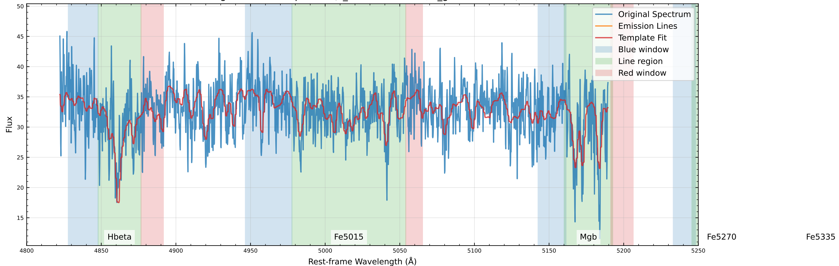
Original Data Comparison (v_star=-13.5 km/s, v_gas=23.1 km/s)
