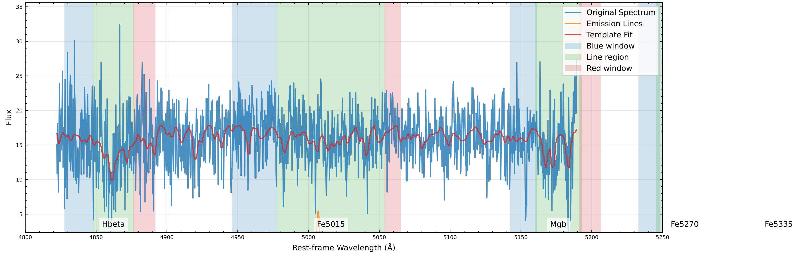
Original Data Comparison (v_star=-24.6 km/s, v_gas=84.0 km/s)
