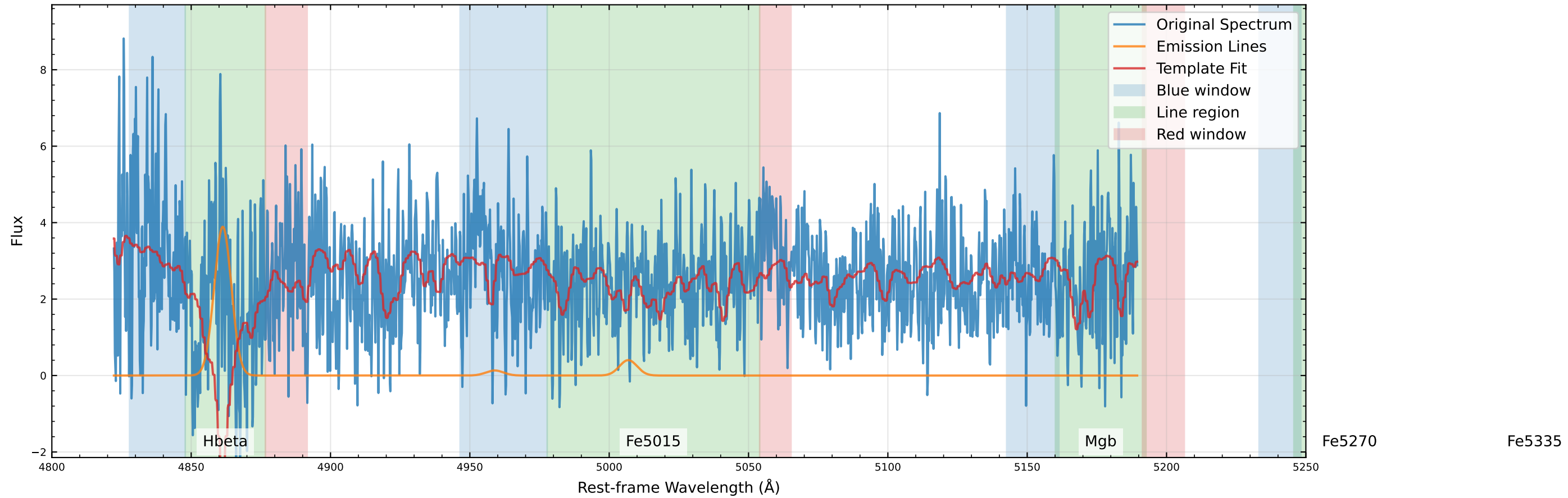
Original Data Comparison (v_star=-9.9 km/s, v_gas=-113.4 km/s)
