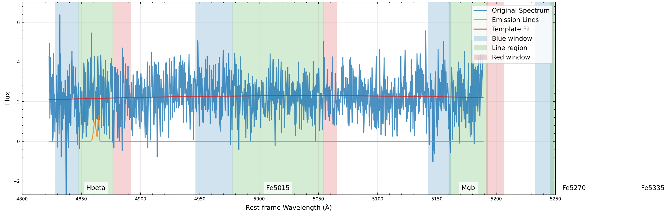
Original Data Comparison (v_star=0.0 km/s, v_gas=-210.5 km/s)
