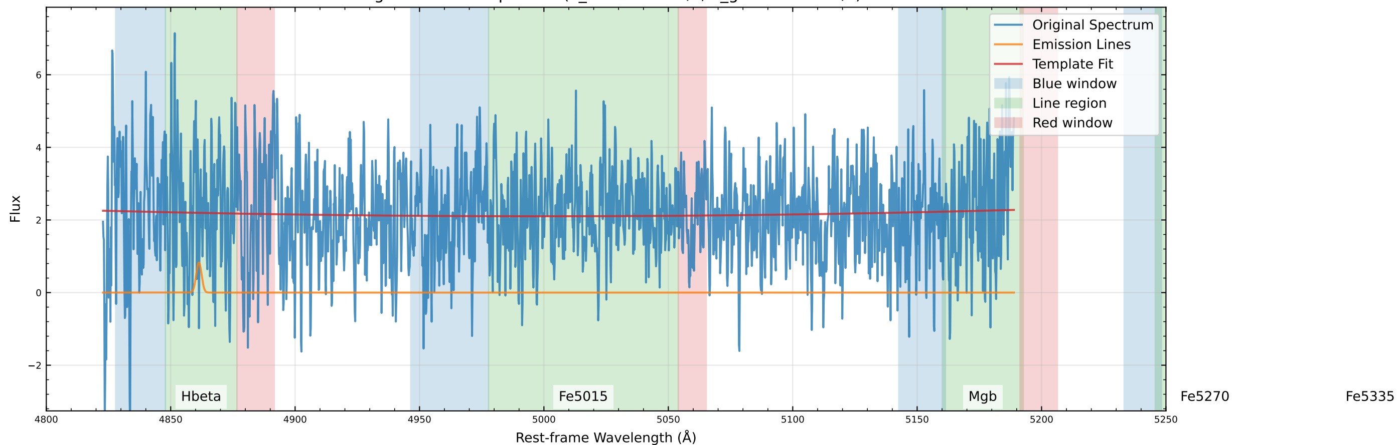
Original Data Comparison (v_star=0.0 km/s, v_gas=-80.2 km/s)
