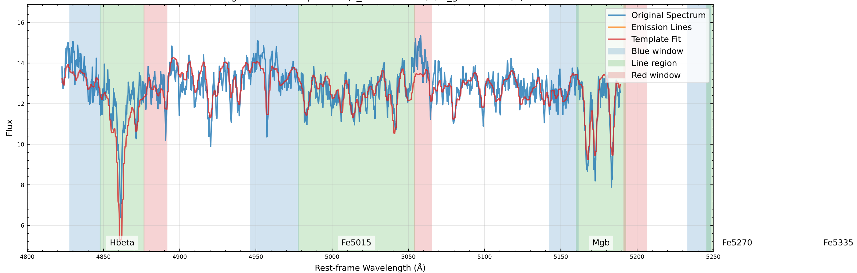
Original Data Comparison ( v_{\text{star}}=-7.3 km/s, v_{\text{gas}}=9.8 km/s)
