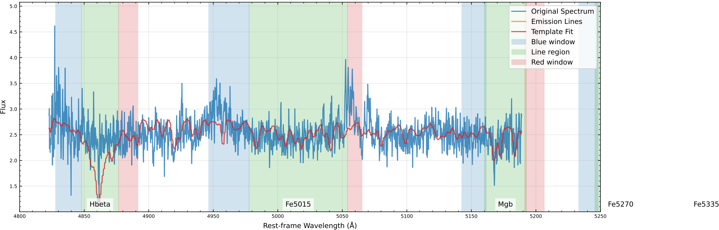
Original Data Comparison (v_star=-83.7 km/s, v_gas=-255.1 km/s)
