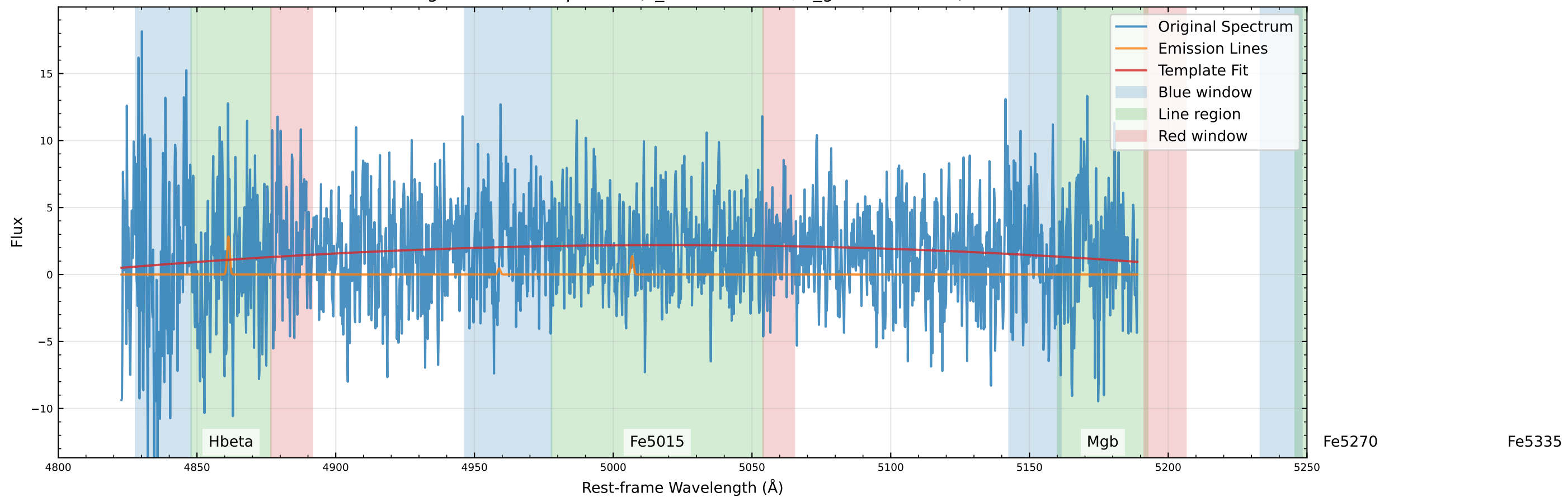
Original Data Comparison (v_star=0.0 km/s, v_gas=10.9 km/s)
