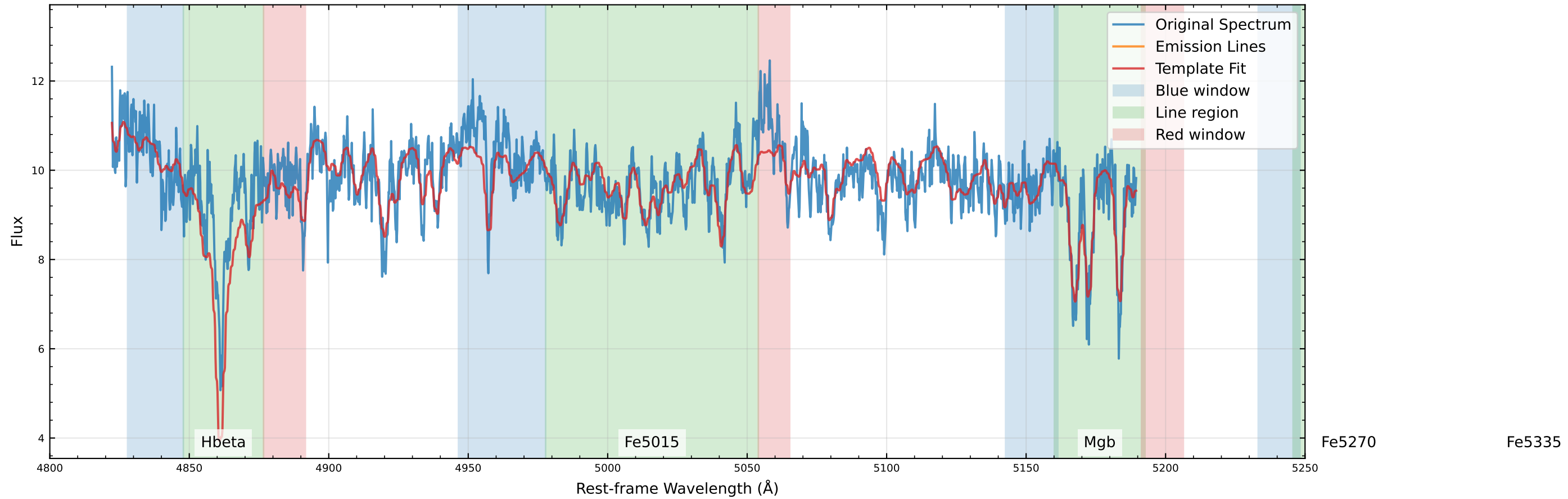
Original Data Comparison (v_star=-6.8 km/s, v_gas=-29.8 km/s)
