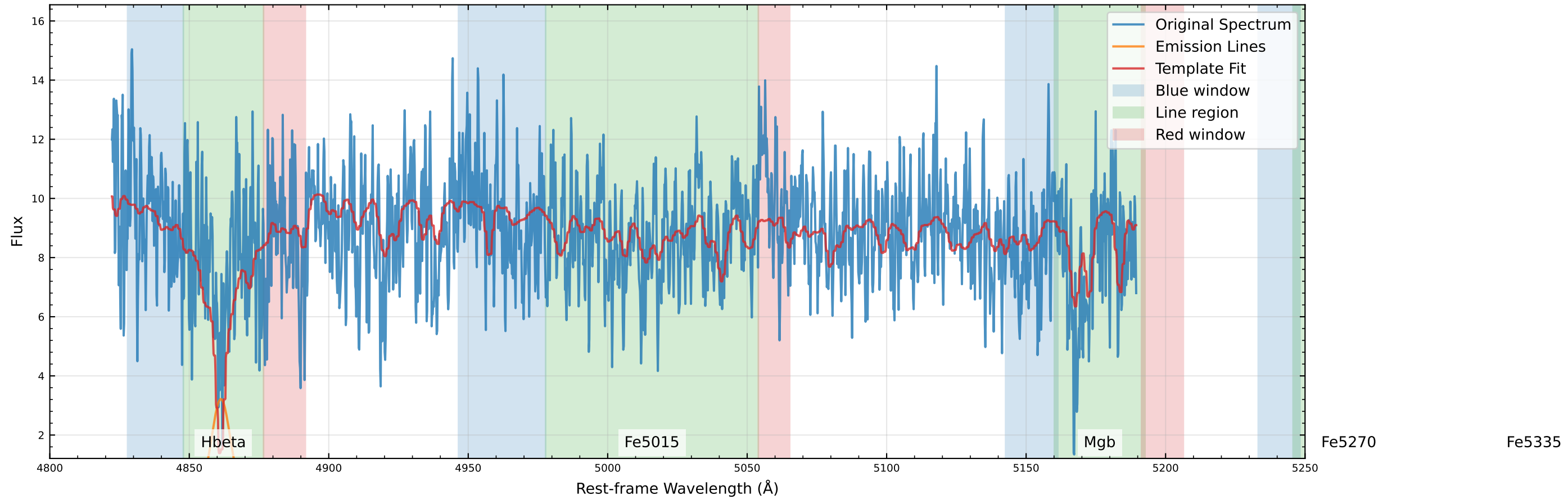
Original Data Comparison (v_star=-17.3 km/s, v_gas=-66.1 km/s)
