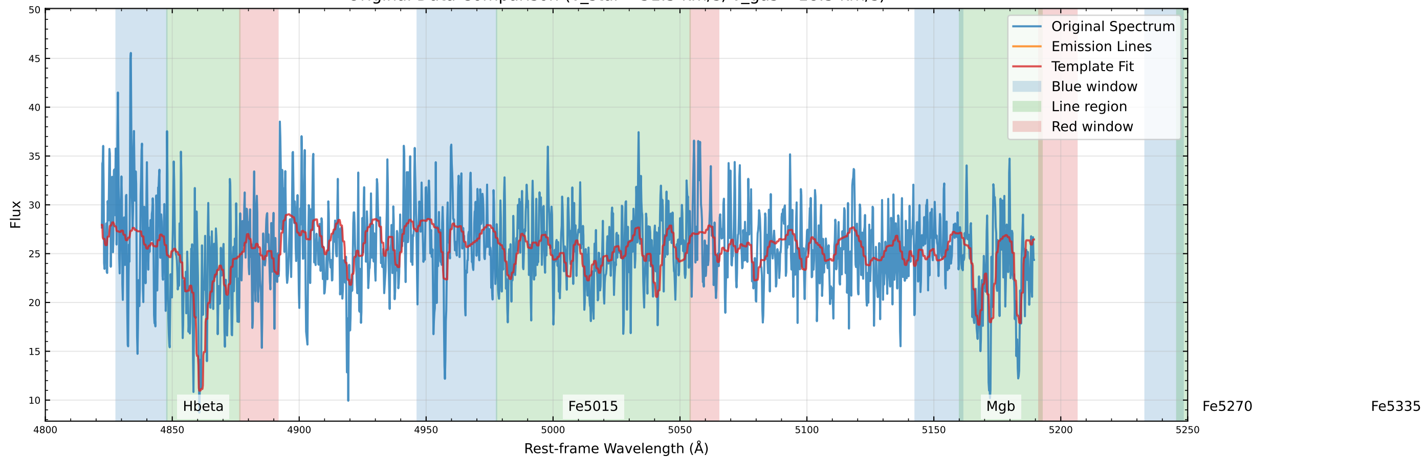
Original Data Comparison (v_star=-31.5 km/s, v_gas=-18.3 km/s)
