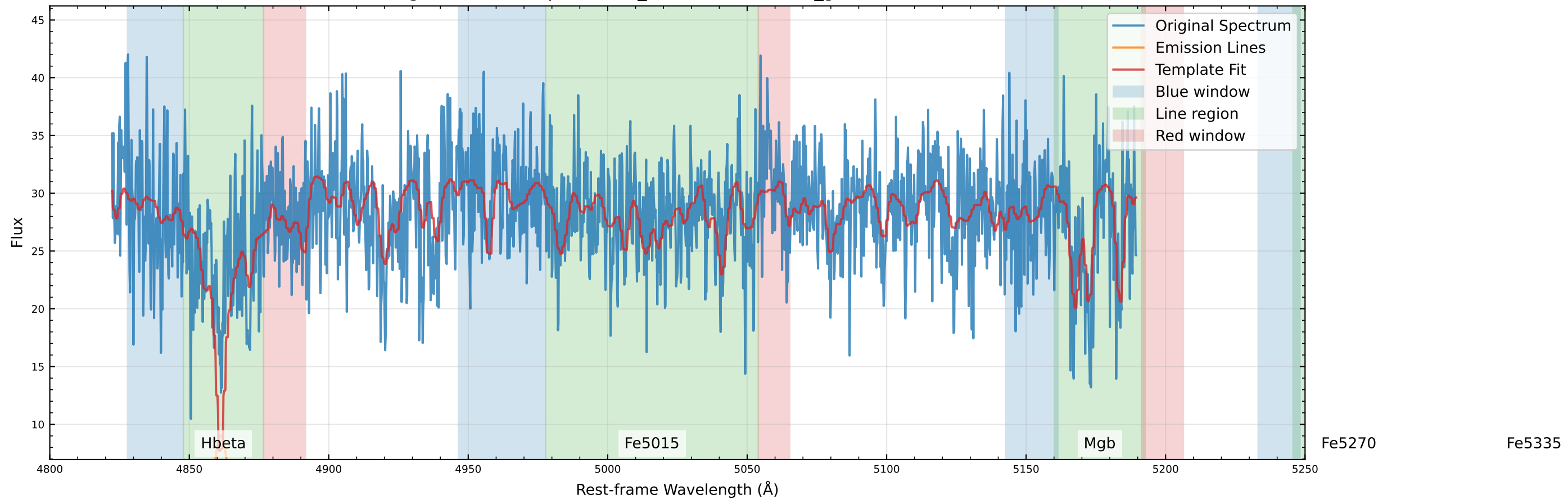
Original Data Comparison (v_star=-21.9 km/s, v_gas=-29.0 km/s)
