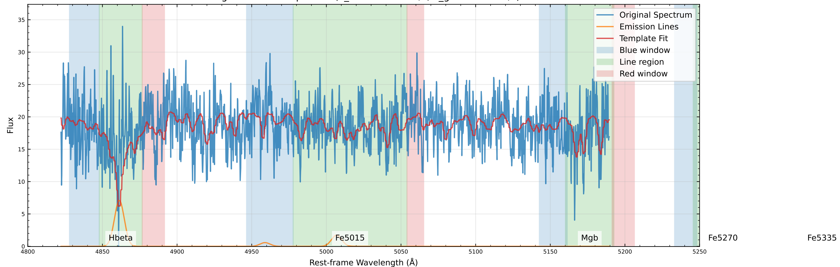
Original Data Comparison (v_star=-34.7 km/s, v_gas=46.0 km/s)
