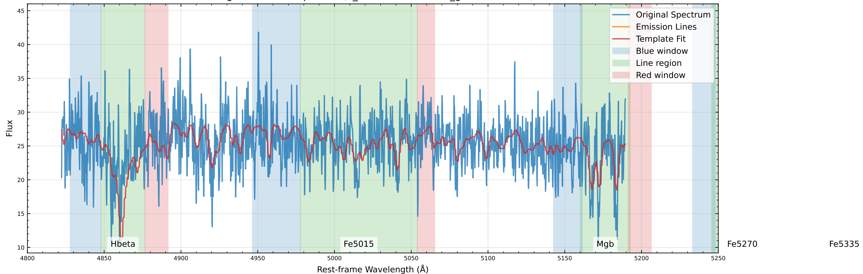
Original Data Comparison (v_star=-17.9 km/s, v_gas=57.9 km/s)
