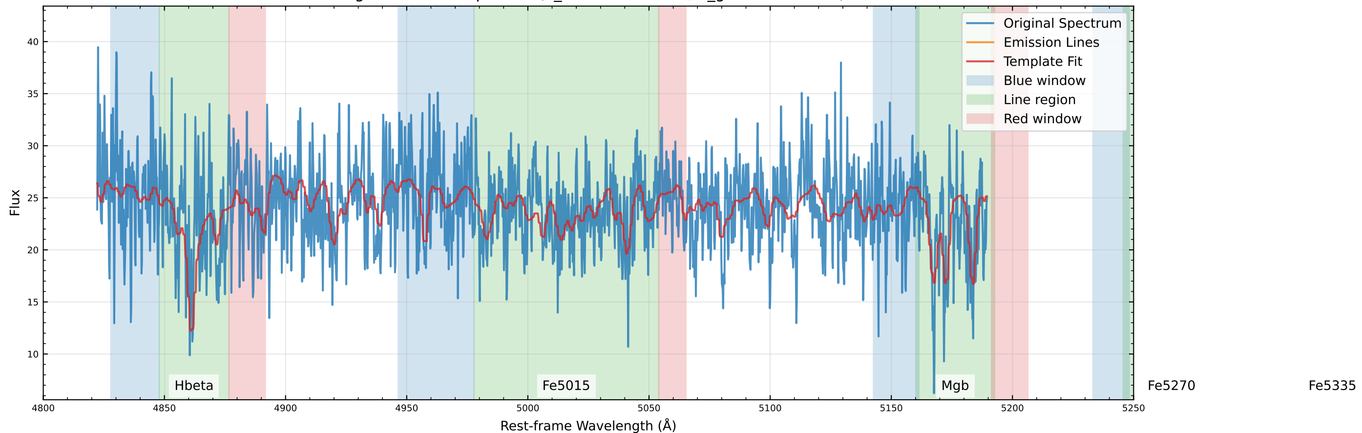
Original Data Comparison (v_star=-15.8 km/s, v_gas=-18.8 km/s)
