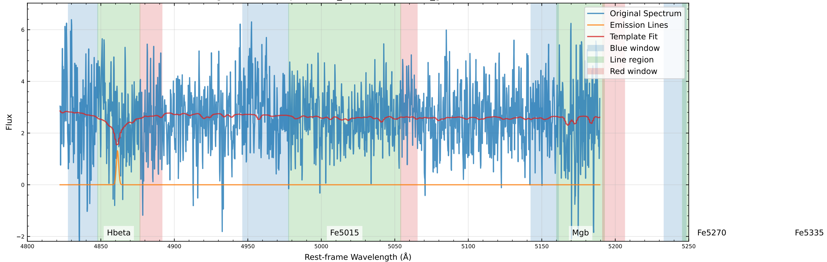
Original Data Comparison ( v_{\text{star}}=-14.0 km/s, v_{\text{gas}}=-33.7 km/s)
