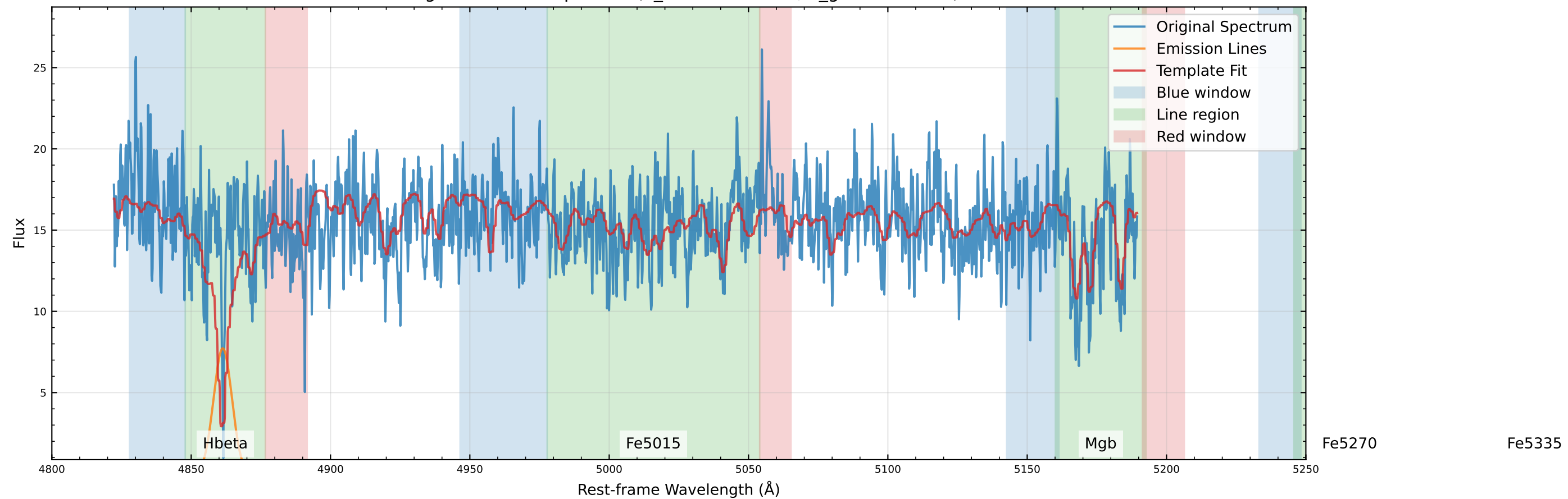
Original Data Comparison (v_star=-3.3 km/s, v_gas=5.3 km/s)
