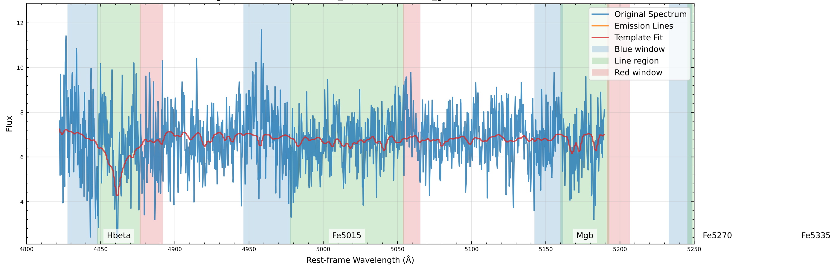
Original Data Comparison (v_star=-51.6 km/s, v_gas=156.8 km/s)
