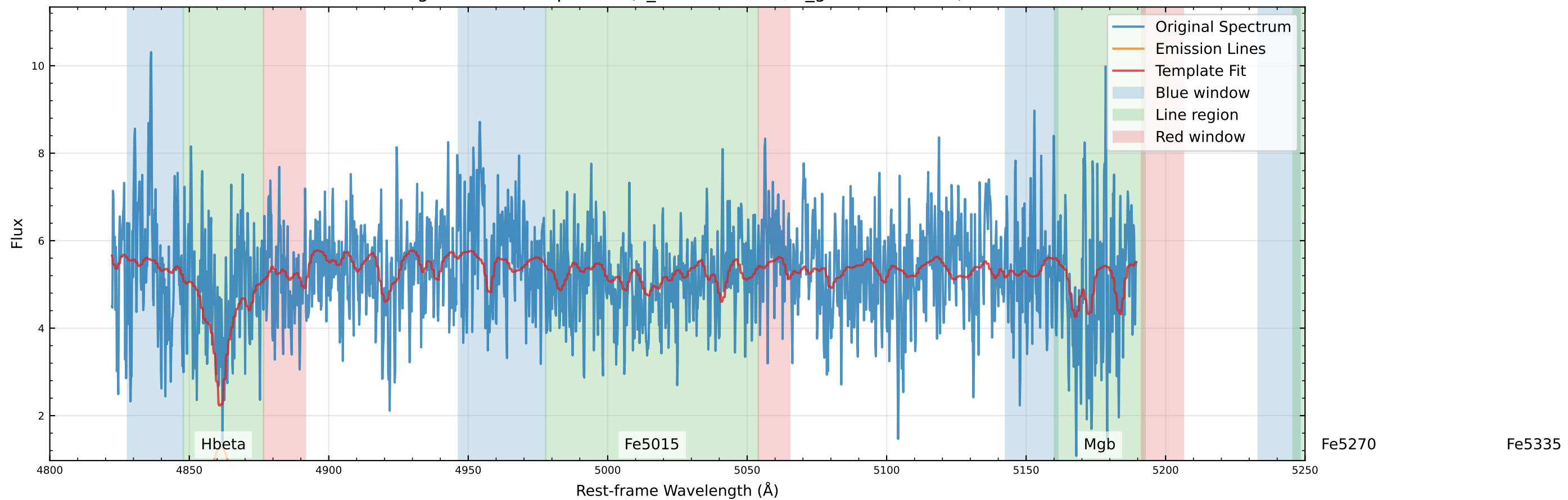
Original Data Comparison (v_star=3.3 km/s, v_gas=-65.0 km/s)
