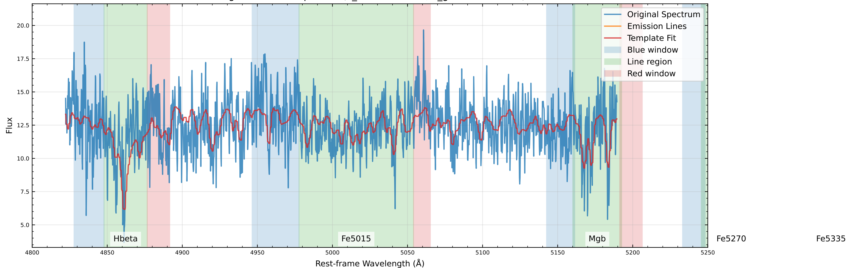
Original Data Comparison (v_star=0.7 km/s, v_gas=192.7 km/s)
