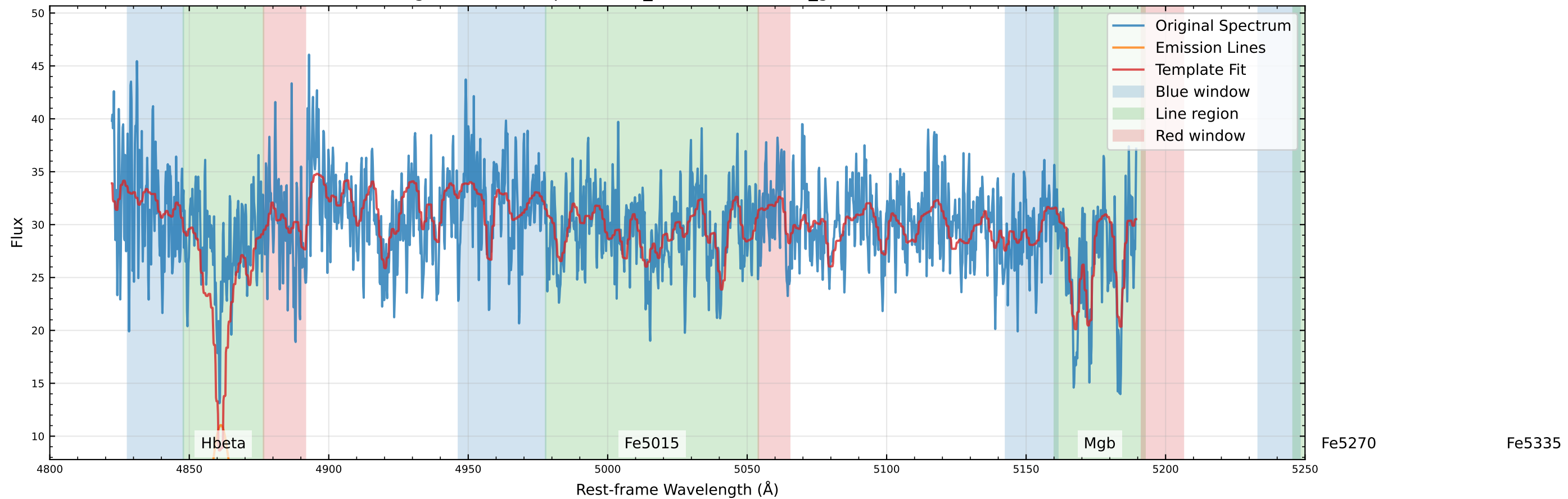
Original Data Comparison (v_star=-9.1 km/s, v_gas=-32.5 km/s)
