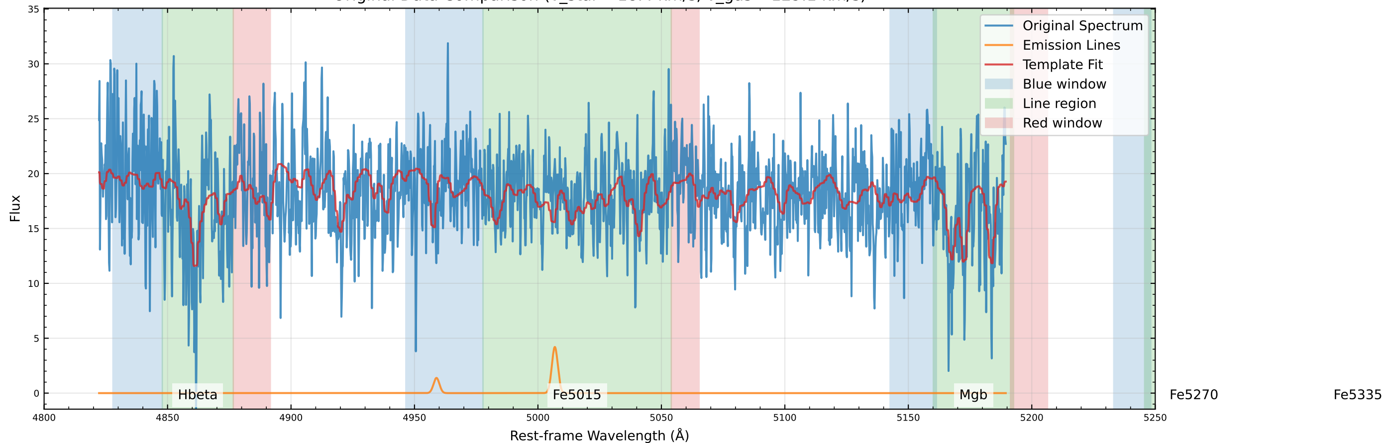
Original Data Comparison (v_star=-18.4 km/s, v_gas=-129.1 km/s)
