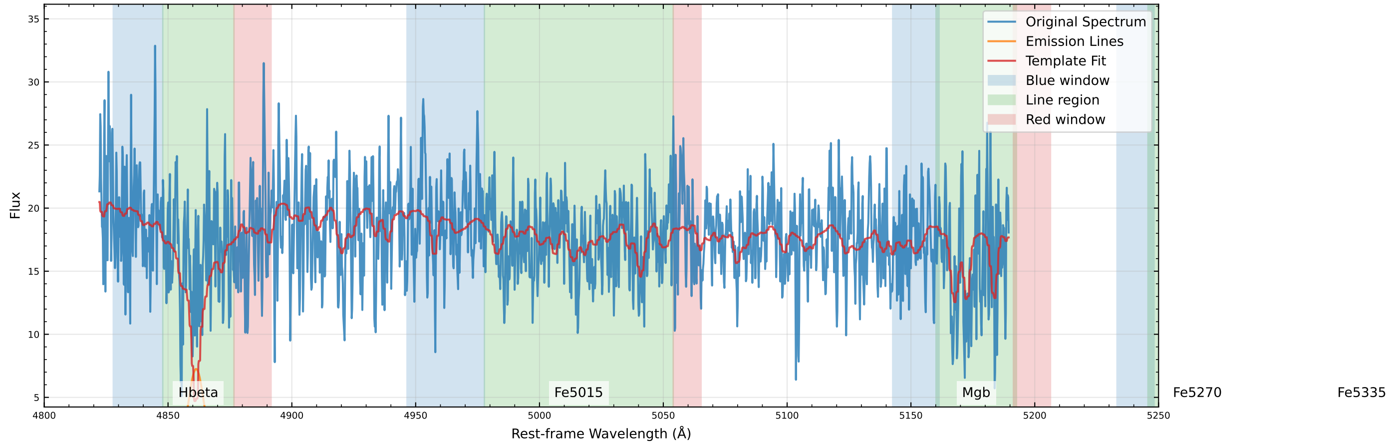
Original Data Comparison (v_star=9.1 km/s, v_gas=47.7 km/s)
