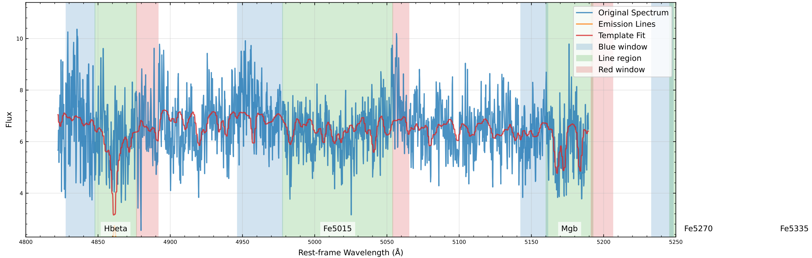
Original Data Comparison (v_star=-15.2 km/s, v_gas=30.7 km/s)
