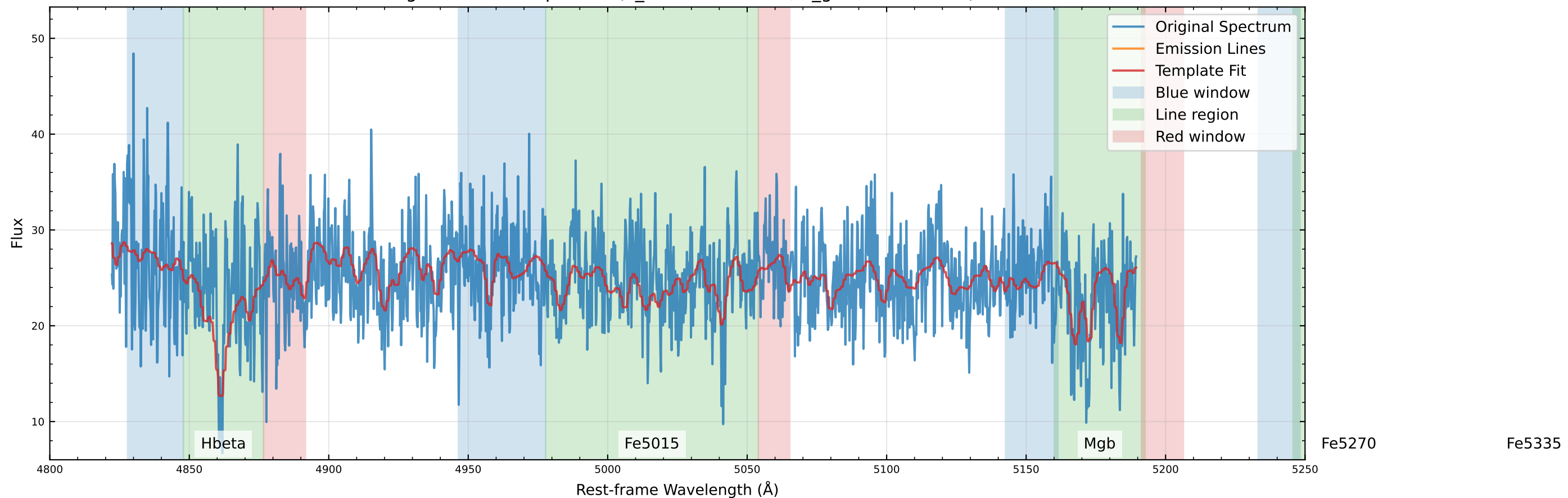
Original Data Comparison (v_star=-19.2 km/s, v_gas=101.2 km/s)
