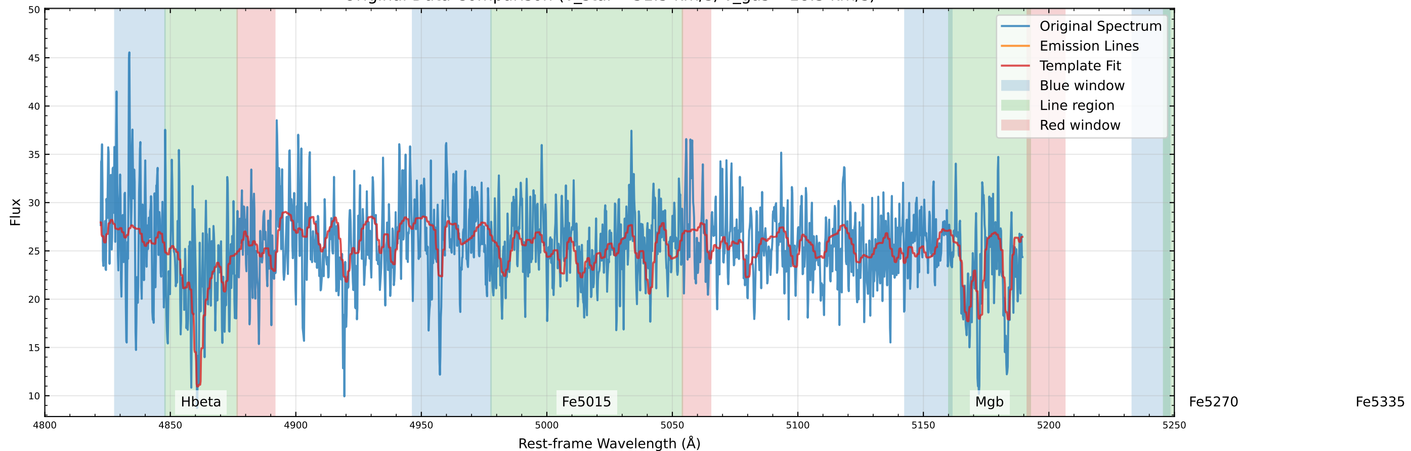
Original Data Comparison (v_star=-31.5 km/s, v_gas=-18.3 km/s)
