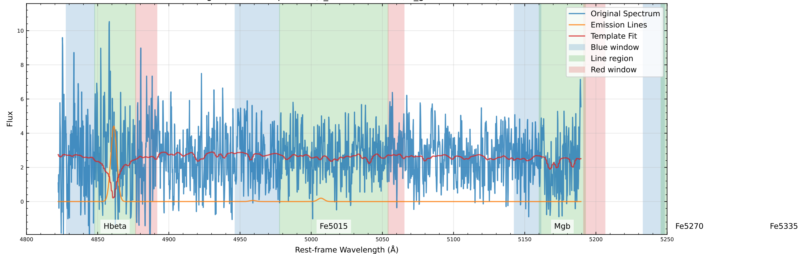
Original Data Comparison (v_star=-36.4 km/s, v_gas=-169.9 km/s)
