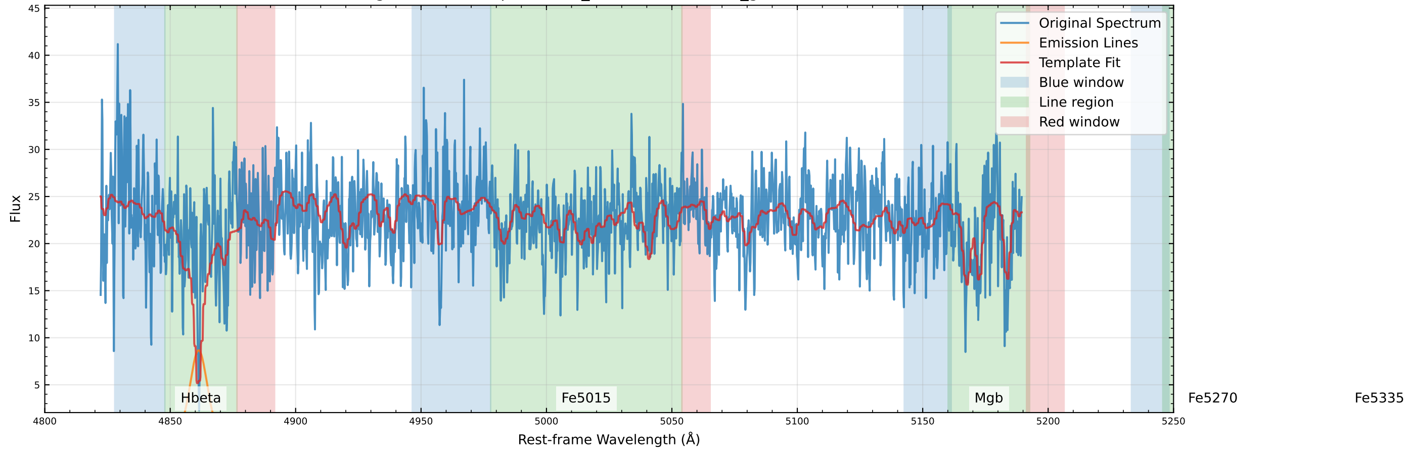
Original Data Comparison (v_star=-17.4 km/s, v_gas=8.8 km/s)
