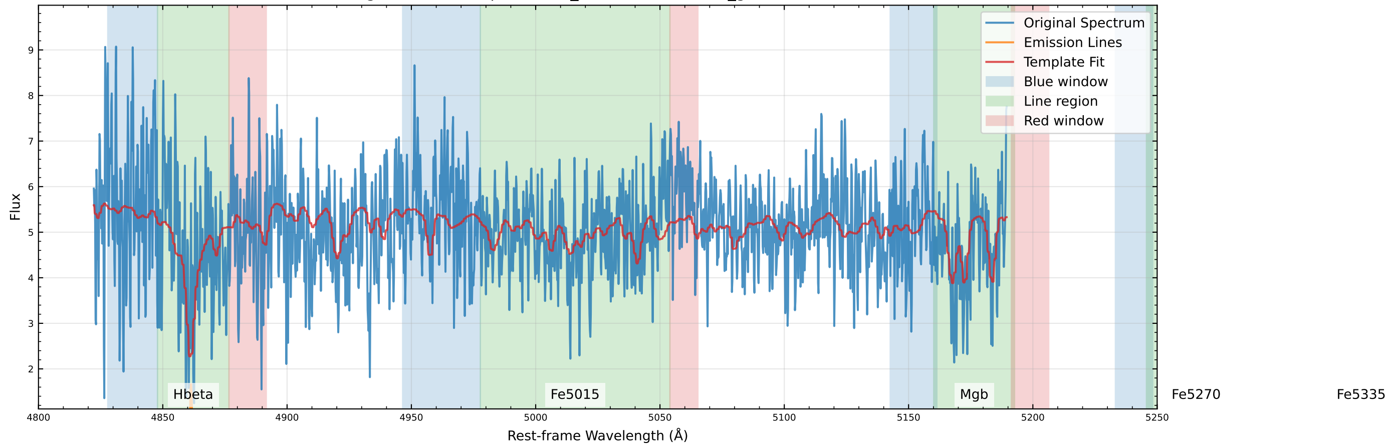
Original Data Comparison (v_star=-10.9 km/s, v_gas=2.5 km/s)
