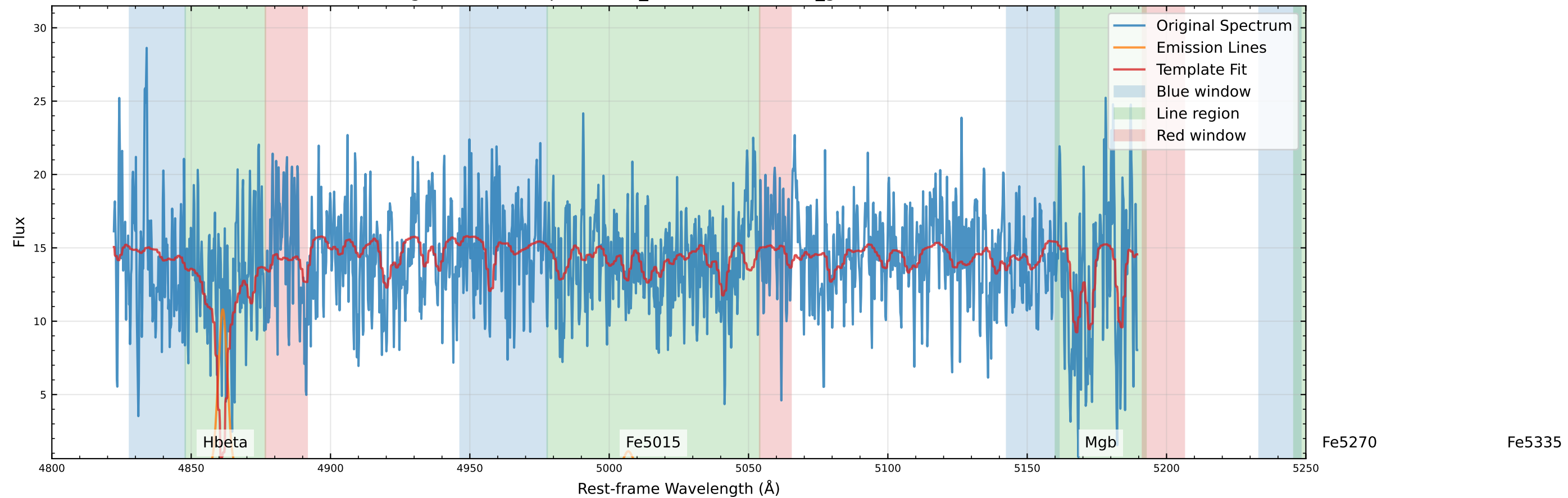
Original Data Comparison ( v_{\text{star}}=-30.7 km/s, v_{\text{gas}}=-60.9 km/s)
