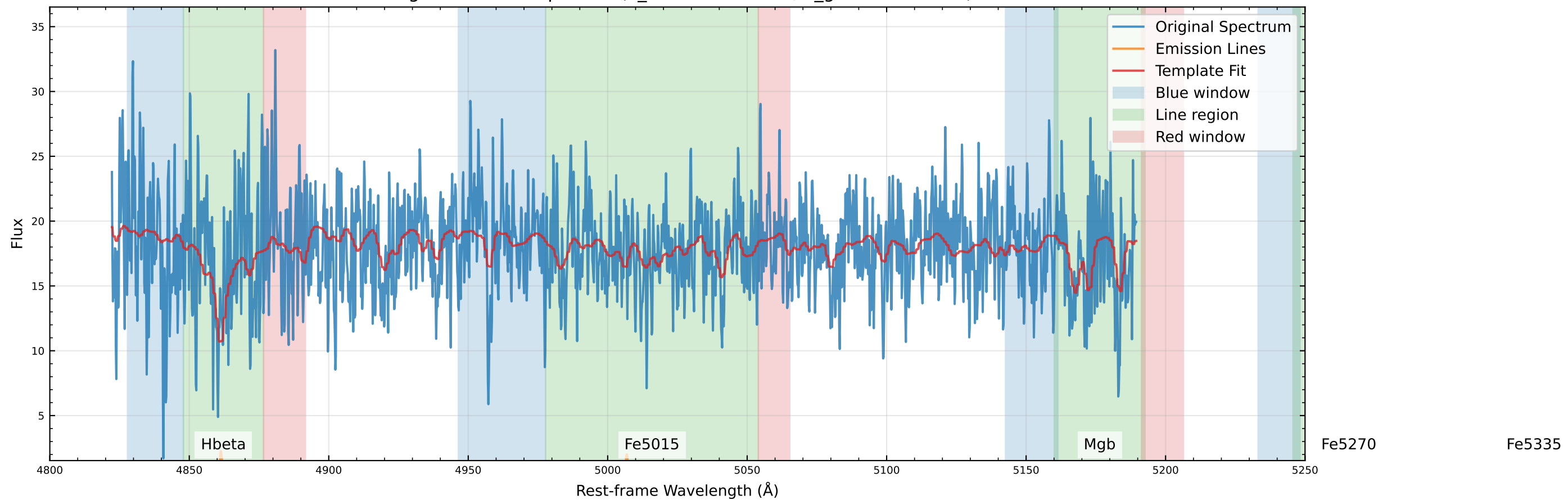
Original Data Comparison (v_star=-36.3 km/s, v_gas=-17.0 km/s)
