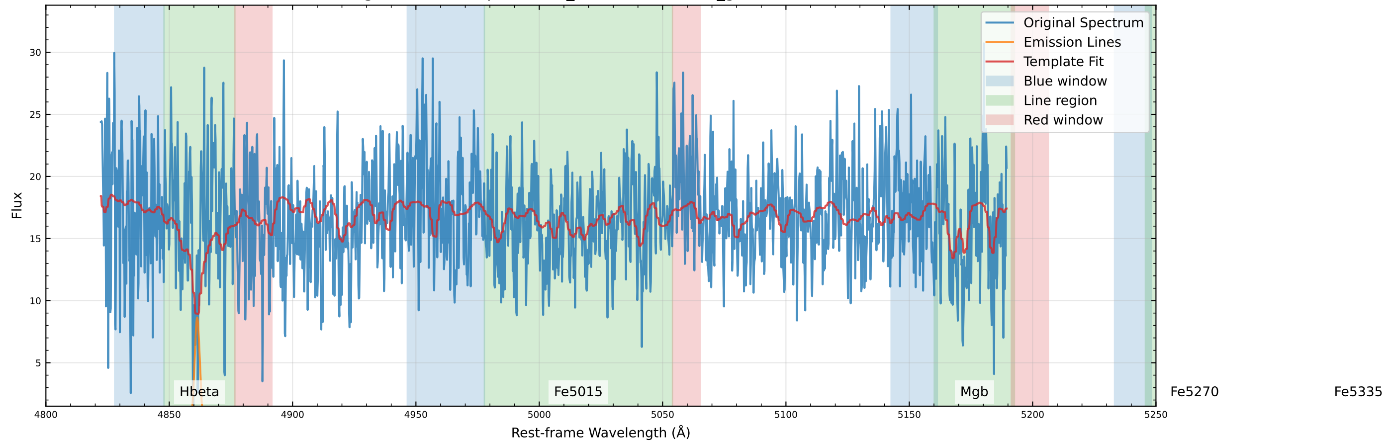
Original Data Comparison (v_star=36.6 km/s, v_gas=136.7 km/s)
