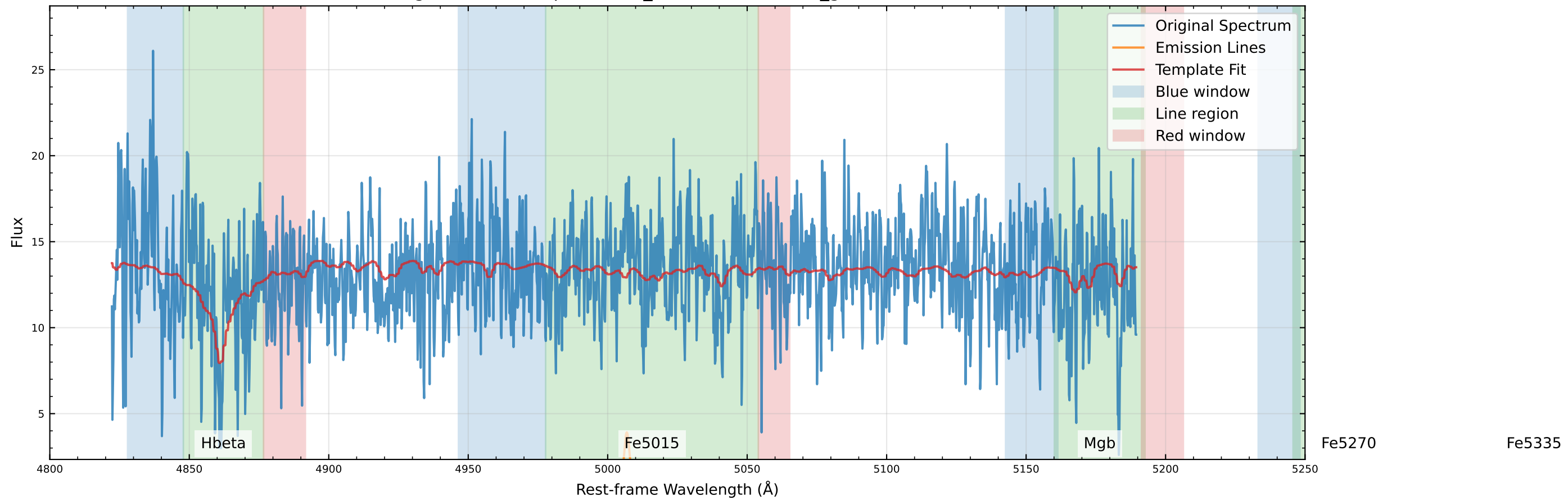
Original Data Comparison (v_star=-39.2 km/s, v_gas=-8.2 km/s)
