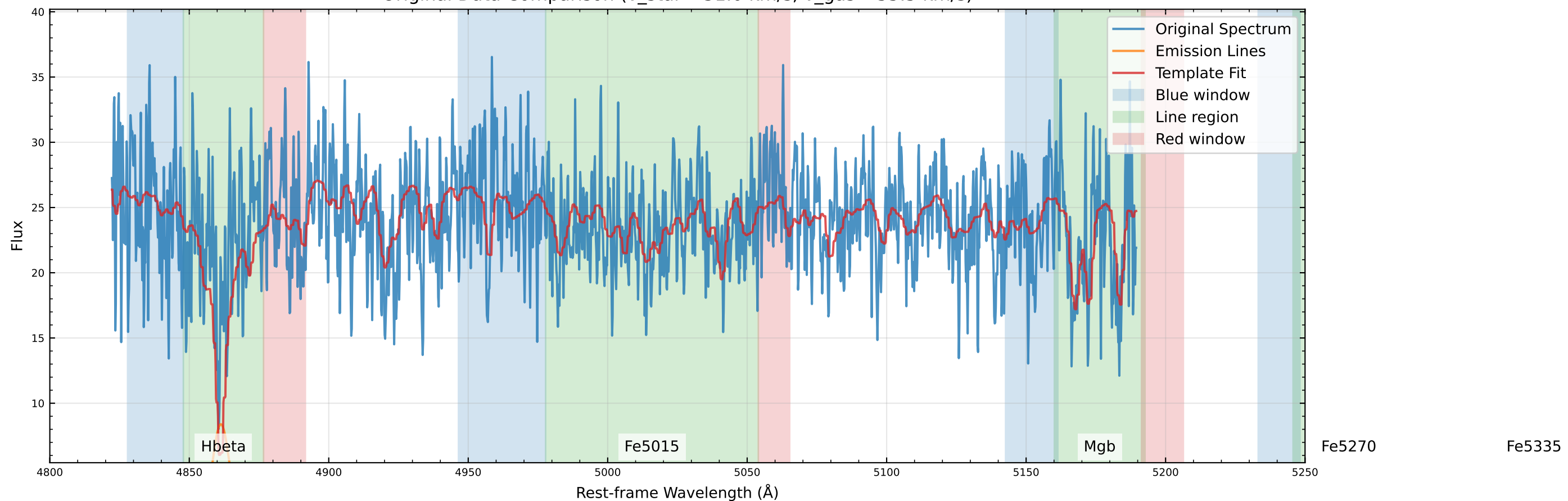
Original Data Comparison (v_star=-31.0 km/s, v_gas=-55.5 km/s)
