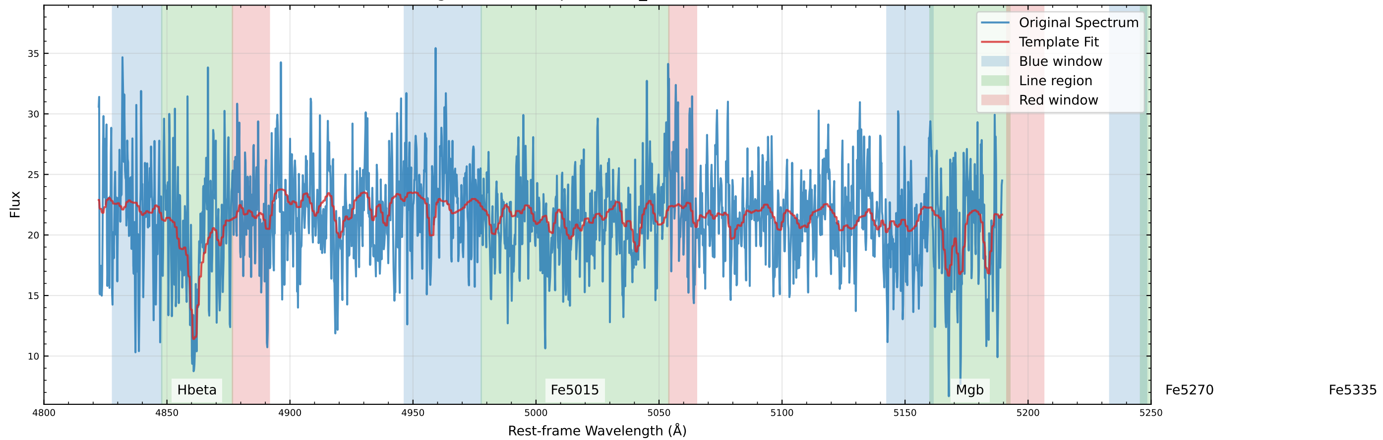
Original Data Comparison (v_star=-20.4 km/s)
